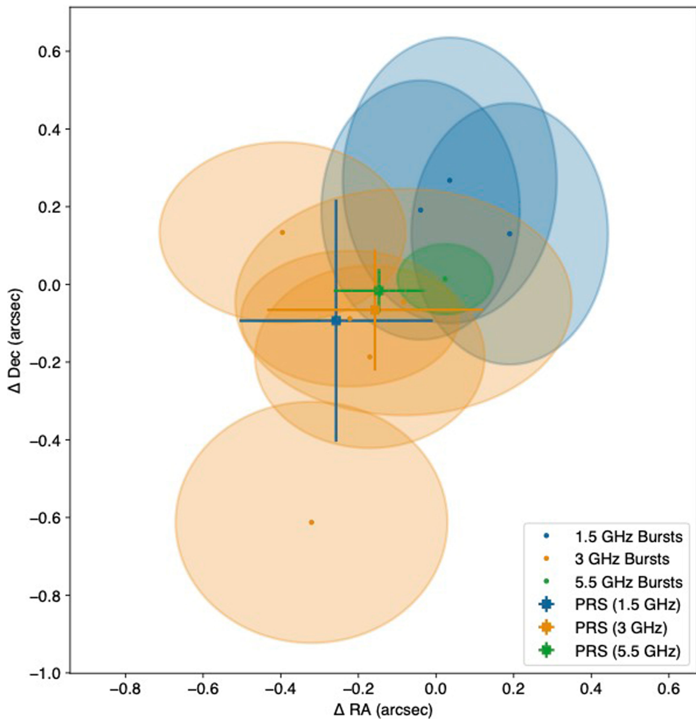
Extended Data Fig. 1 | Positions of the bursts and persistent radio source identified with VLA observations. The observations were performed at 1.5, 3, and 5.5 GHz. They were shown as offsets from the best-fit position of the ensemble of bursts, at RA = 16h02m04.272s, dec. = -11° 17' 17.32" (J2000). The
